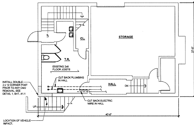
1 BASEMENT REMOVAL PLAN SCALE: 1/8" = 1'-0"
