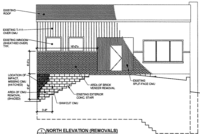
3 NORTH ELEVATION (REMOVALS) SCALE: 1/8" = 1'-0"
