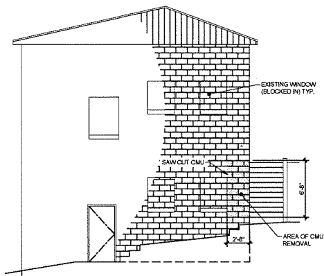
2 EAST ELEVATION (REMOVALS) SCALE: 1/8" = 1'-0"
