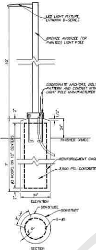
LIGHT POLE DETAIL NOT TO SCALE
