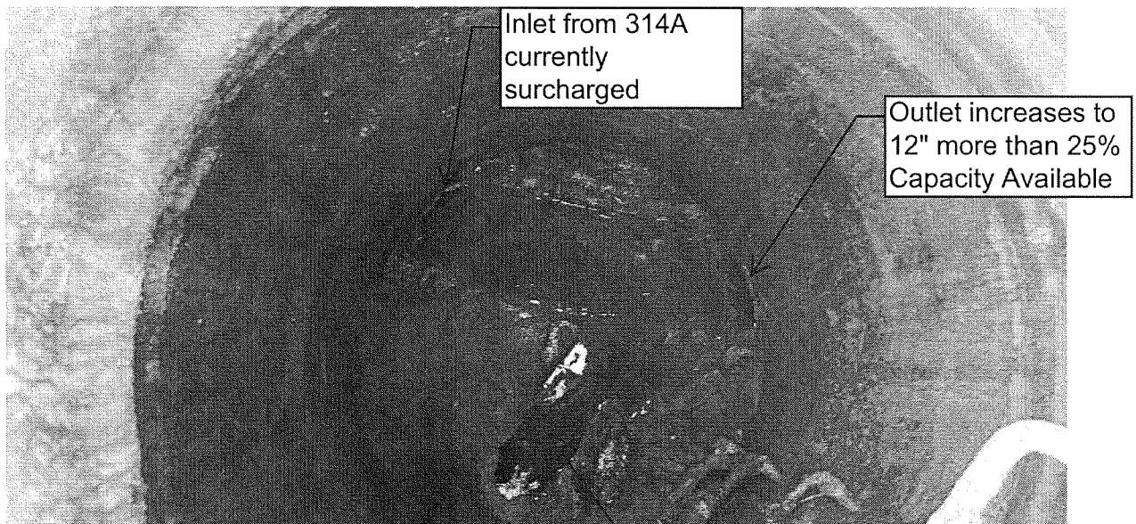
Manhole 314 – Adequate Capacity pipe sizes increase to 12"
