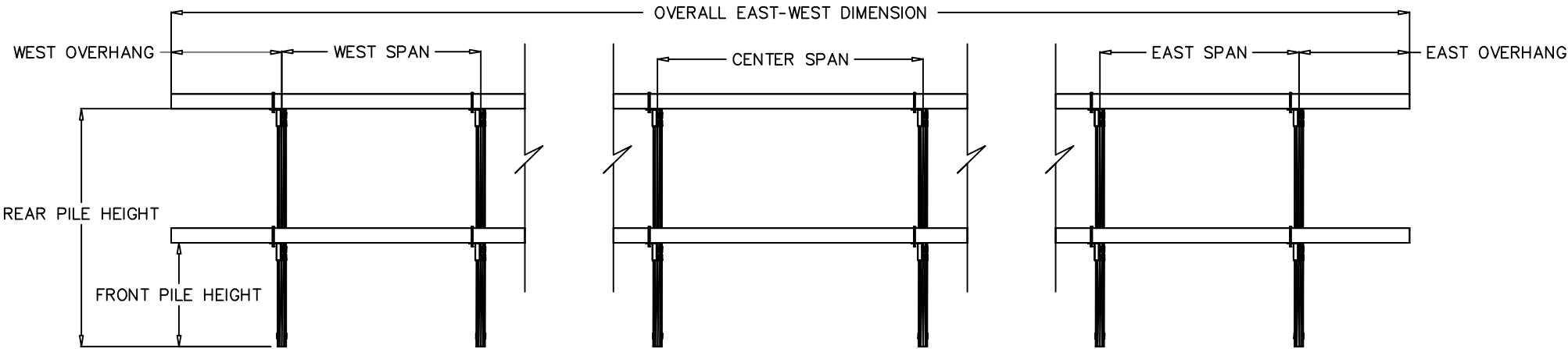
PILE SPACING ELEVATION
