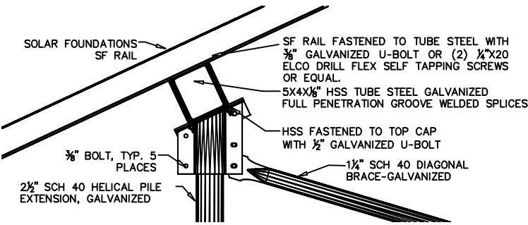
LOWER CAP DETAIL
